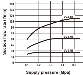
Max. Suction flow function
