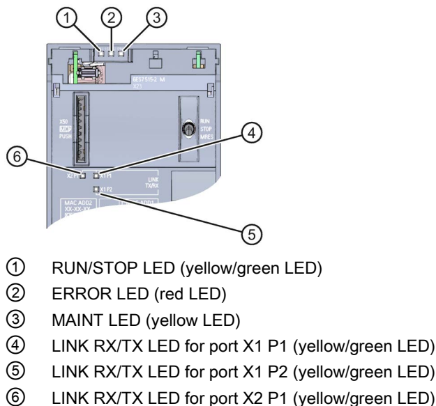
Figure 4-1 LED display of the CPU 1515-2 PN (without front panel)
