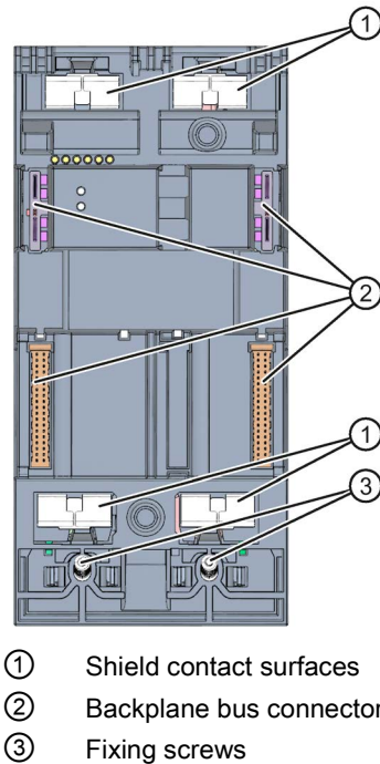
Figure 2-5 View of the CPU 1515-2 PN - rear
